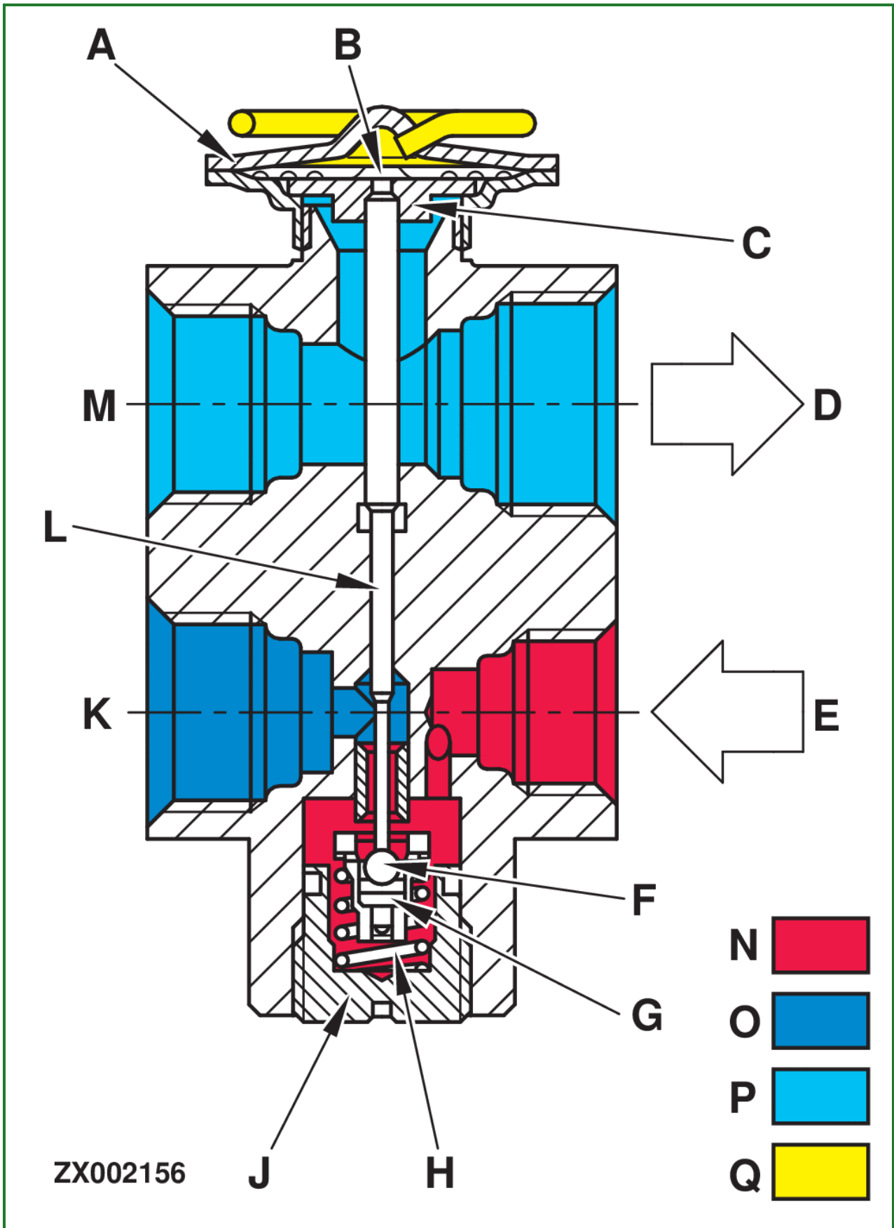
LX002156-UN: Expansion valve operation
