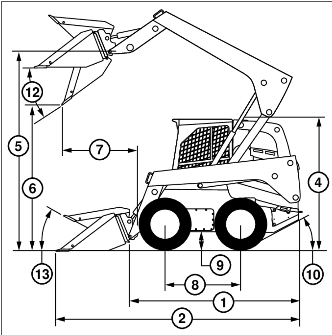
TX1065132-UN: Machine Dimensions-Side View
