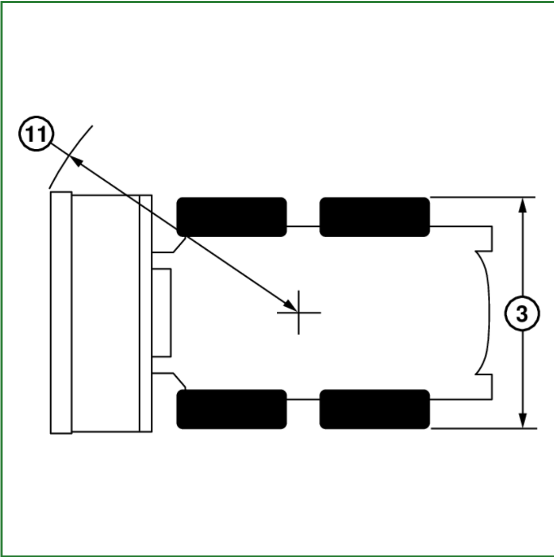
TX1065133-UN: Machine Dimensions-Top View
