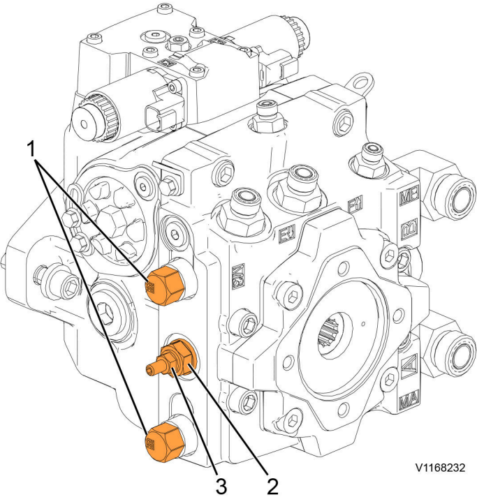
Figure 1 Vibration pump tightening torques
