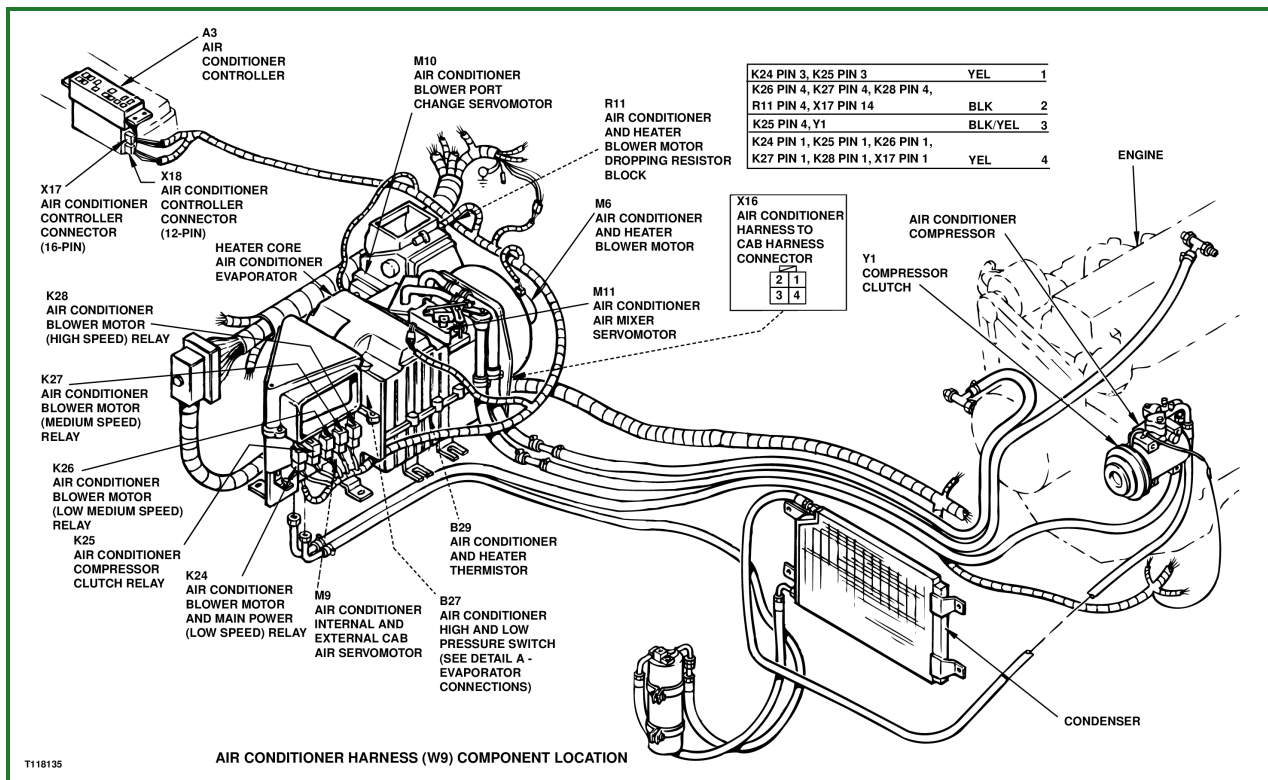
T118135-19: Air Conditioner Harness (W9) Component Location
