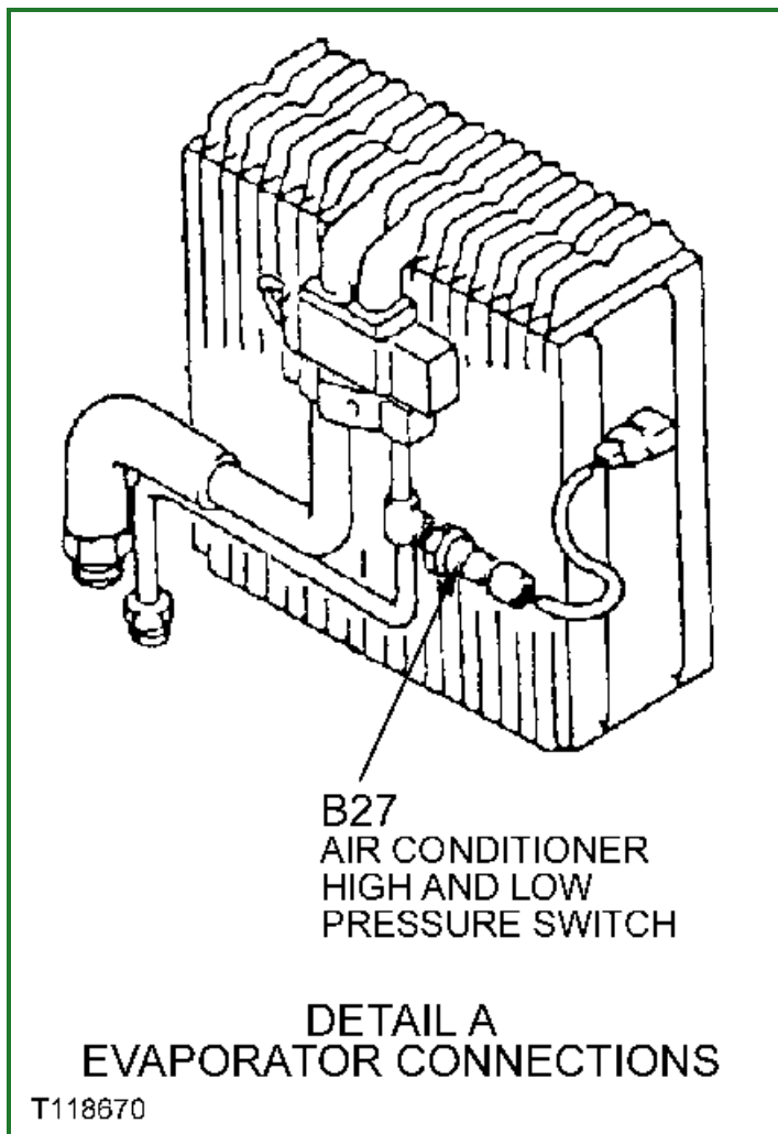
T118670-19: Air Conditioner Harness (W9) Component Location--Detail A
