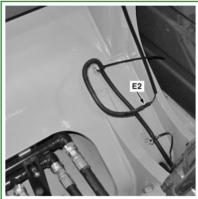
TX1205231A-UN: Boom Light
