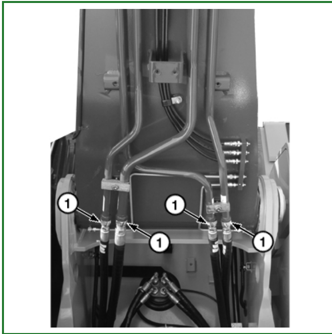
TX1165205A-UN: Boom Hydraulic Lines
